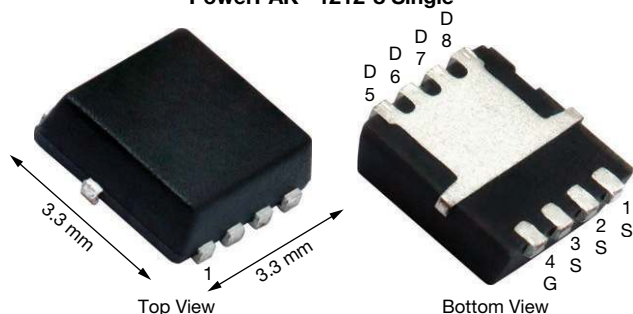
PowerPAK® 1212-8 Single
