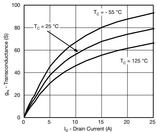
Transconductance
