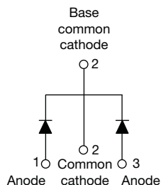
VS-25CTQ...S-M3
