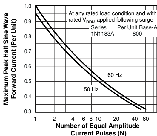
Fig. 10 - Maximum Non-Repulsive Surge Current vs. Number of Current Pulses, 1N1183A Series
