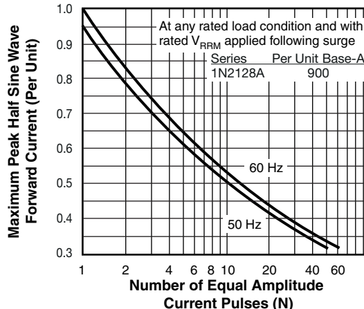
Fig. 11 - Maximum Non-Repulsive Surge Current vs. Number of Current Pulses, 1N2128A Series
