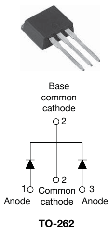
VS-15CTQ...-1PbF
