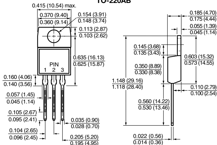
TO-220AB
