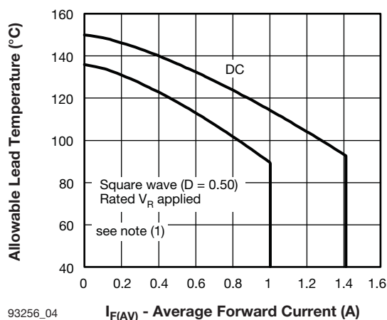
93256_04 I F(AV) - Average Forward Current (A) Fig. 4 - Typical Allowable Lead Temperature vs. Average Forward Current
