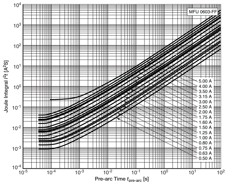
Typical I^2 t vs. t_{pre-arc} characteristic of MFU 0603 (1)
