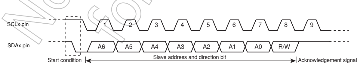
Figure 14-5 Generating the Start Condition and a Slave Address
