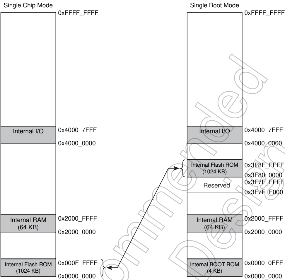
Figure 22-3 Memory Maps for TMPM361F10FG
