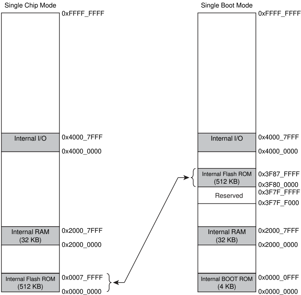
Figure 17-3 Memory Maps for TMPM330FDFG
