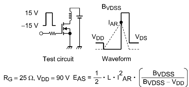
Fig. 8.16 Test Circuit/Waveform
