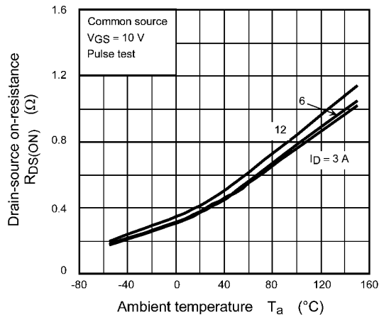
Fig. 8.7 R_{DS(ON)} - T_a
