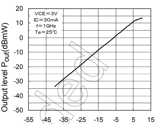
P_{out} - P_{in}
