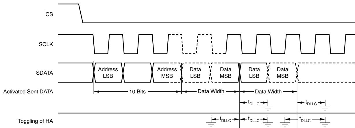
Figure 9. Continuous Write Mode Timing
