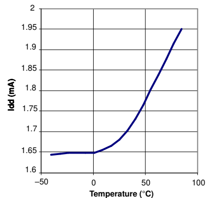
CONVERSION SUPPLY CURRENT vs TEMPERATURE
