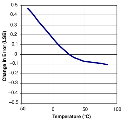
CHANGE IN OFFSET ERROR vs TEMPERATURE
