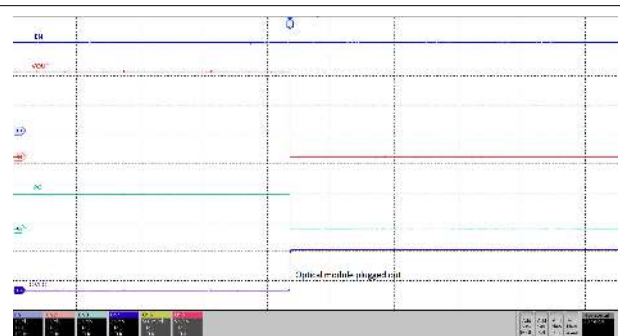
Figure 8-11. Output Voltage Profile When Optical Module is Plugged Out
