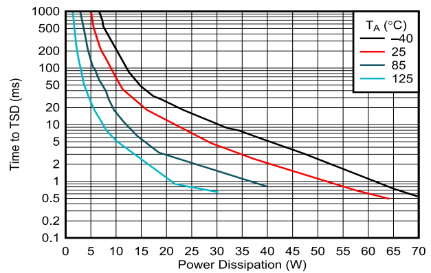
Figure 6-27. Time to Thermal Shutdown During Steady-State
