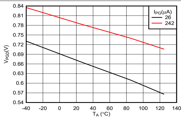
Figure 6-22. PG Pin Voltage vs Temperature (V IN = 0V)
