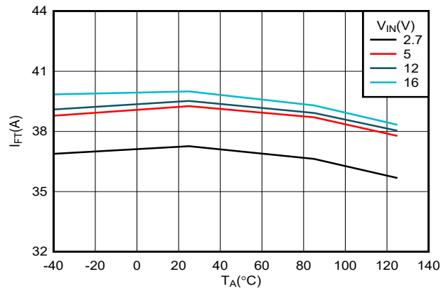
Figure 6-16. Fixed Fast-Trip Threshold vs Temperature
