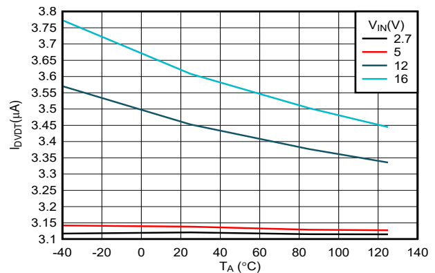
Figure 6-21. DVDIT Charging Current vs Temperature
