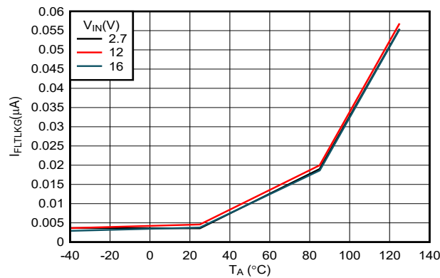
Figure 6-24. FLT Pin Leakage Current vs Temperature
