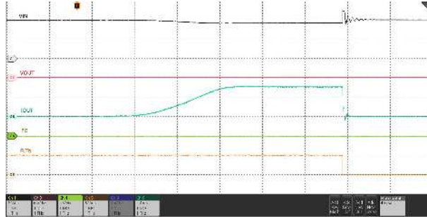
Figure 6-38. Power Up into Short Circuit
