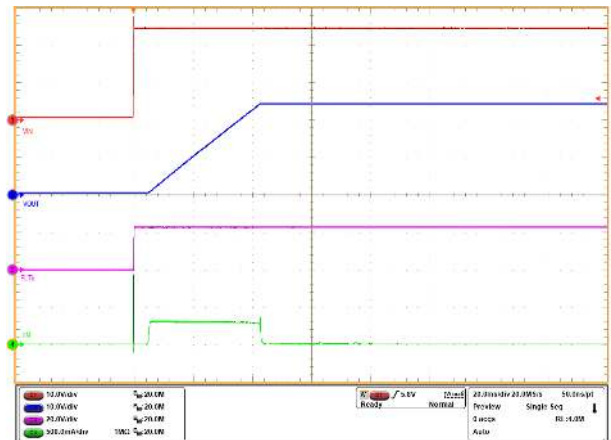
Figure 8-3. Inrush Current Control for Hot Plug-in at Input
