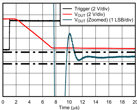
Figure 6-36. Glitch Impulse, Falling Edge, 1-LSB Step
