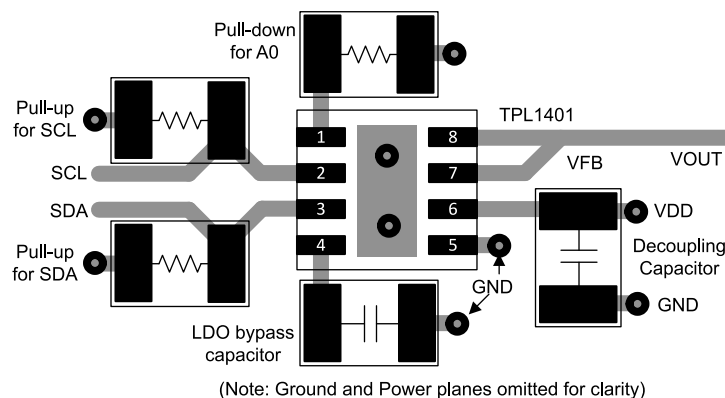
Figure 10-1. Layout Example
