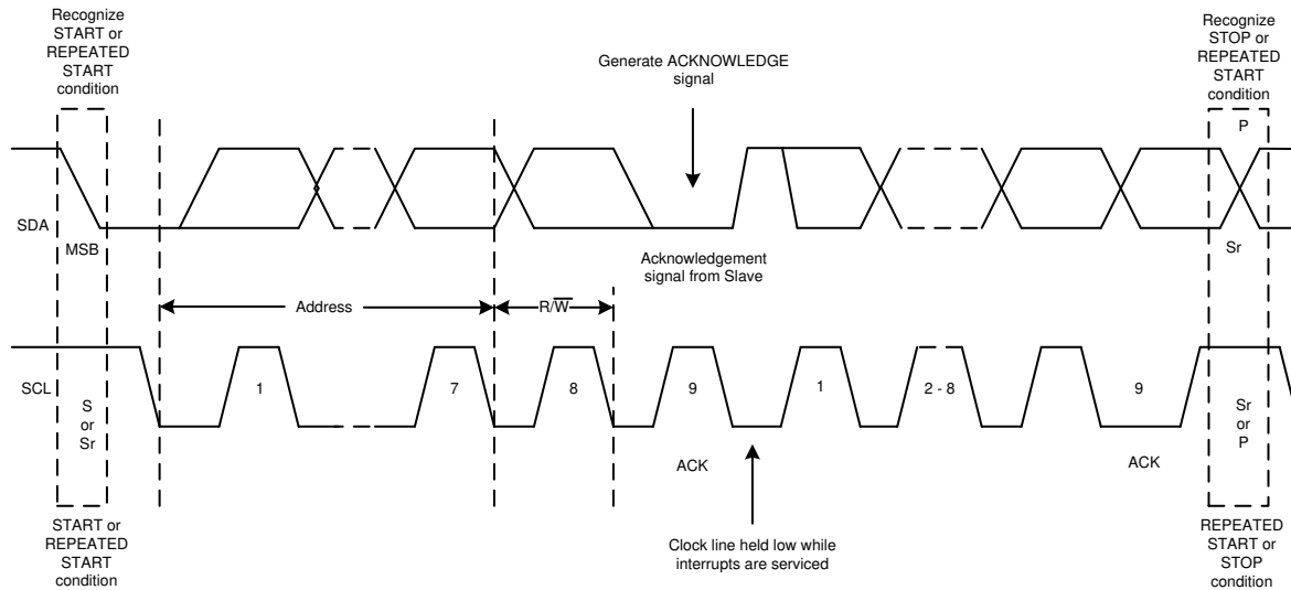
Figure 7-5. I 2 C Bus Protocol
