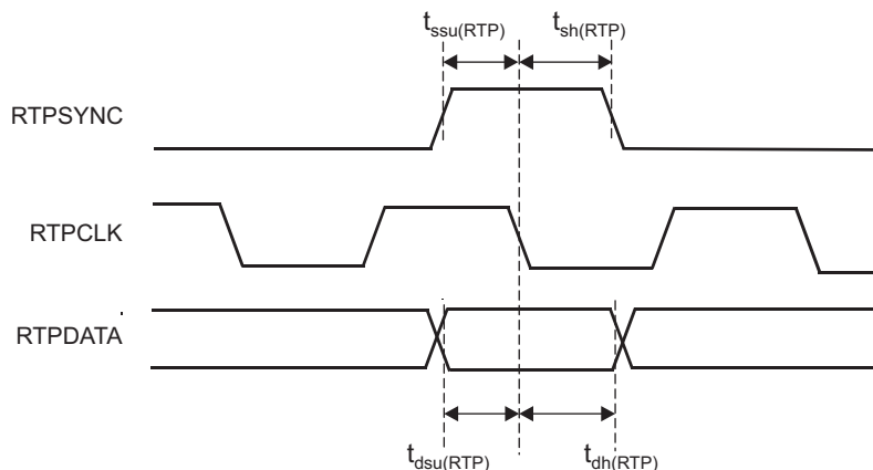
Figure 6-33. RTPDATA Timing
