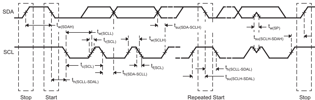
Figure 7-18. I2C Timings
