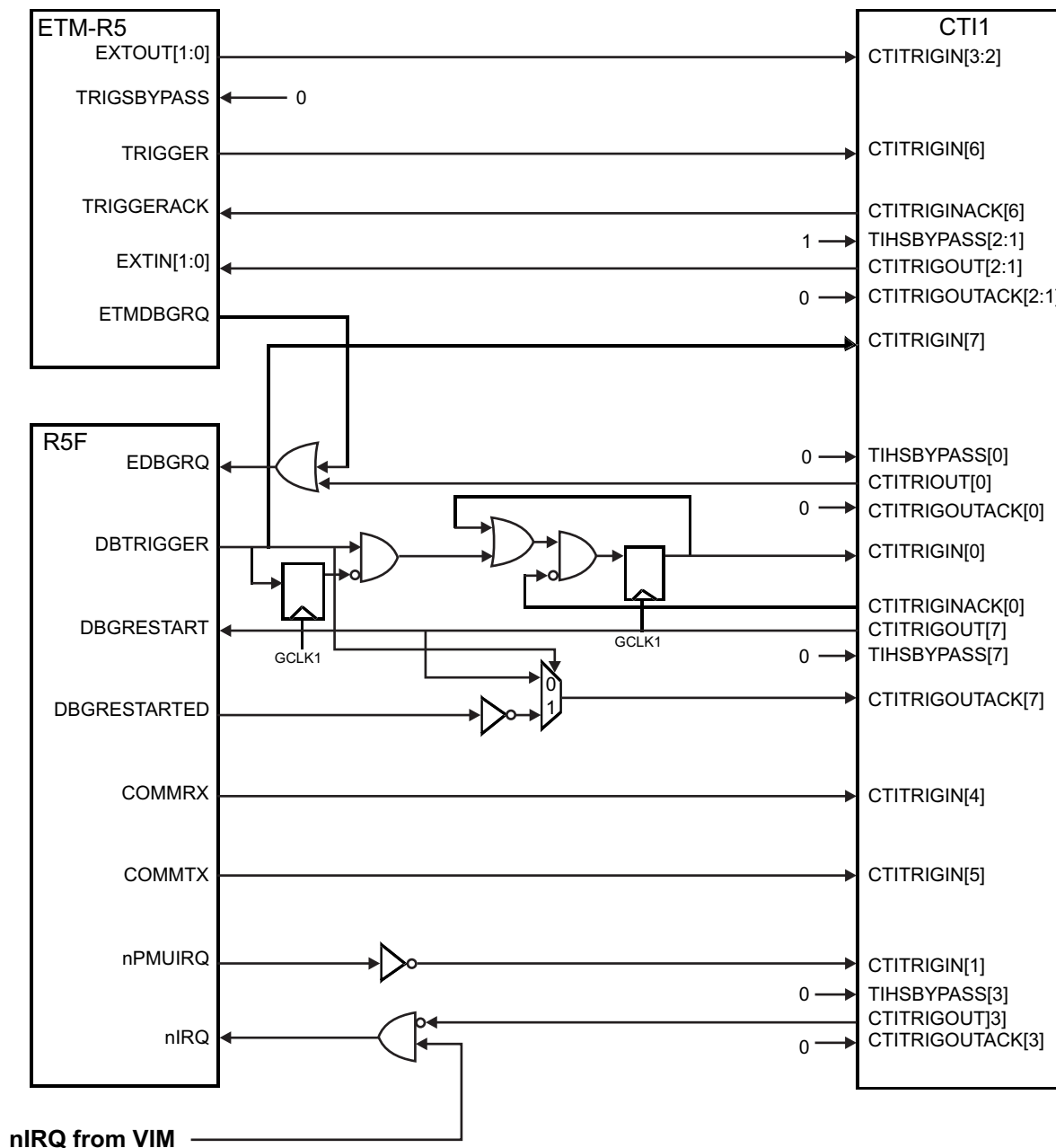
Figure 6-25. CTI1 Mapping
