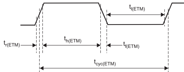
Figure 6-30. ETMTRACECLKOUT Timing
