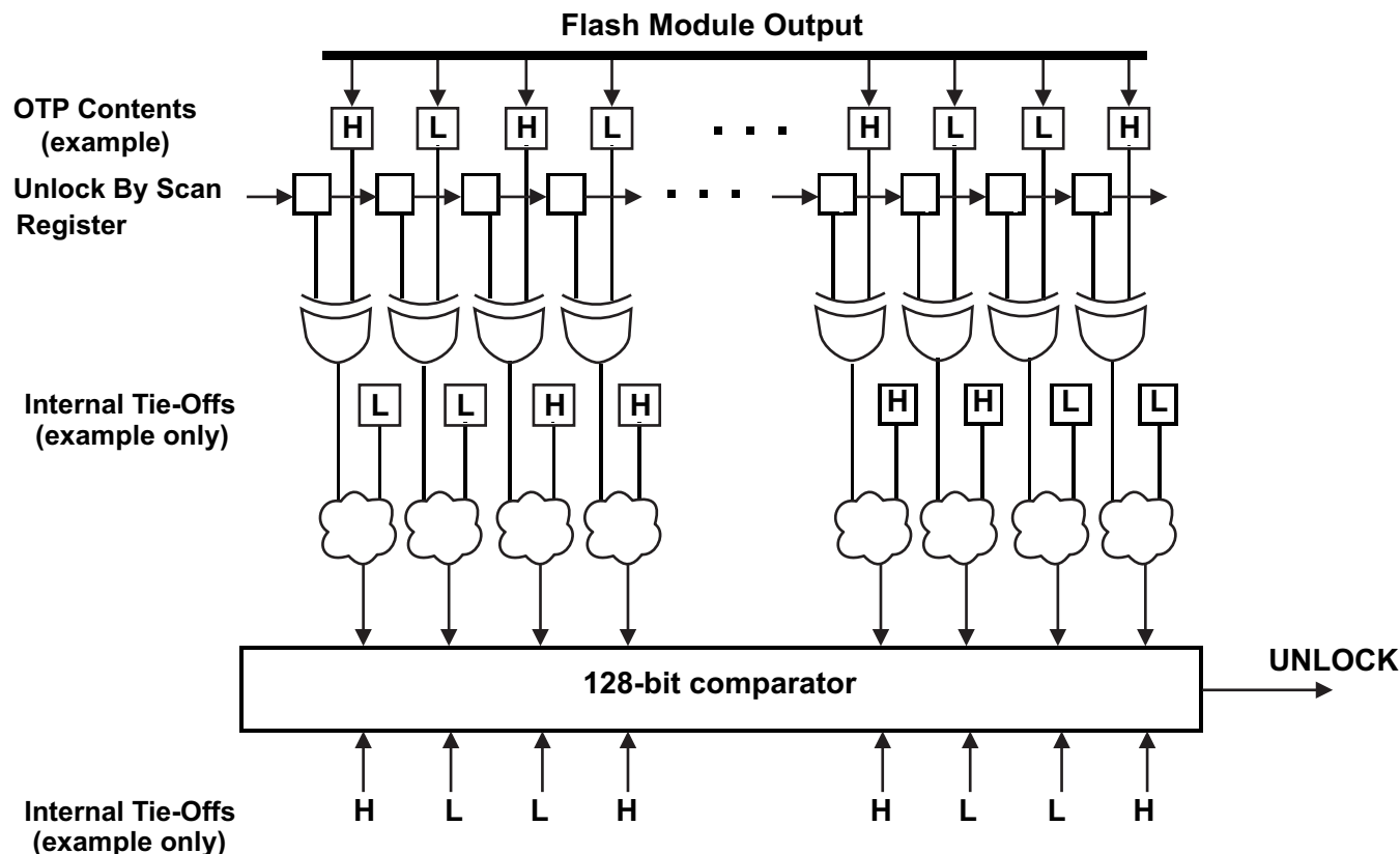
Figure 6-29. AJSM Unlock
