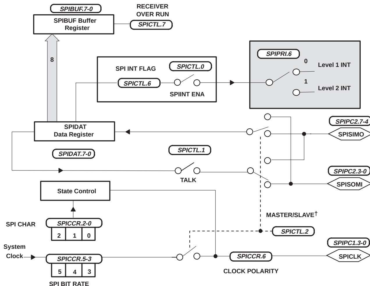
Figure 6. SPI Block Diagram
