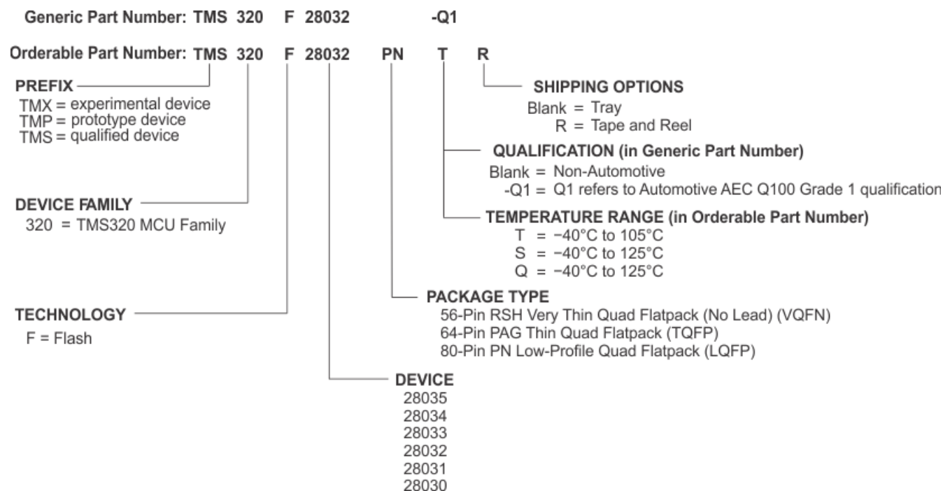
Figure 9-1. Device Nomenclature
