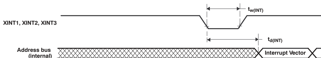
Figure 7-14. External Interrupt Timing
