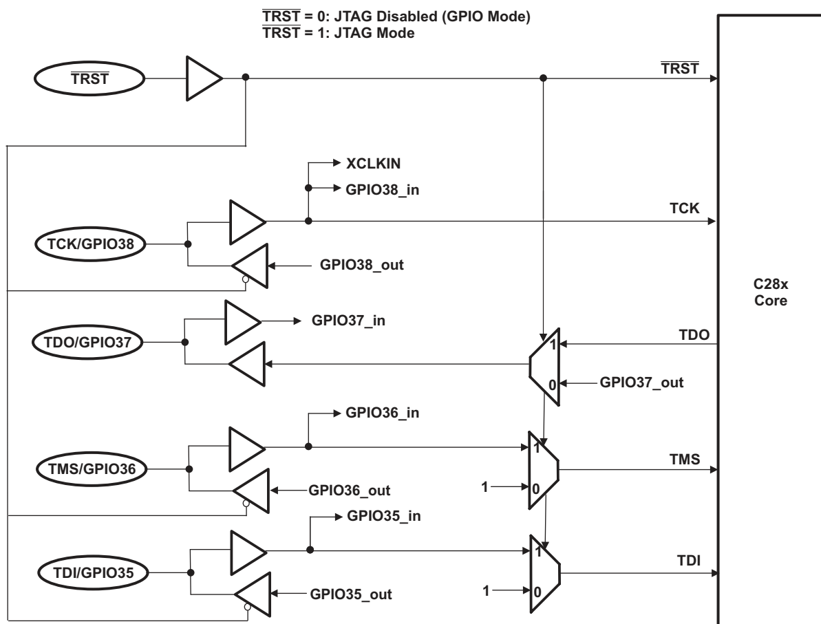
Figure 7-44. JTAG/GPIO Multiplexing
