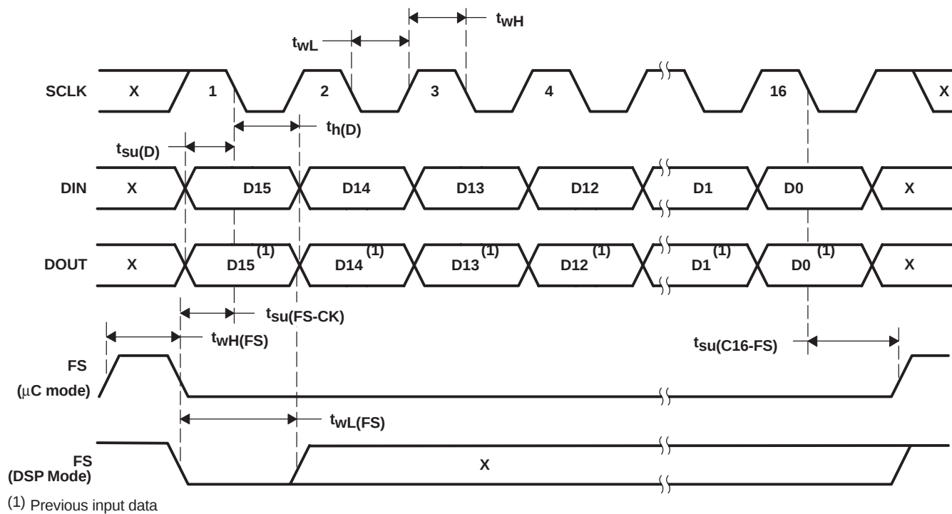
Figure 9. Serial Interface Timing
