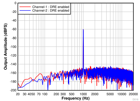
Figure 7-19. FFT With a -60-dB Input With DRE Enabled
