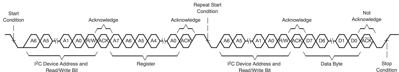
Figure 8-69. I 2 C Single-Byte Read Transfer
