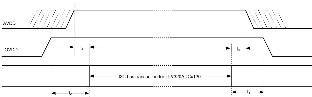
Figure 10-1. Power-Supply Sequencing Requirement Timing Diagram
