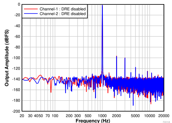
Figure 7-21. FFT With a -1-dB Input With DRE Disabled
