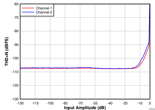
Figure 7-9. THD+N vs Input Amplitude With DRE Disabled
