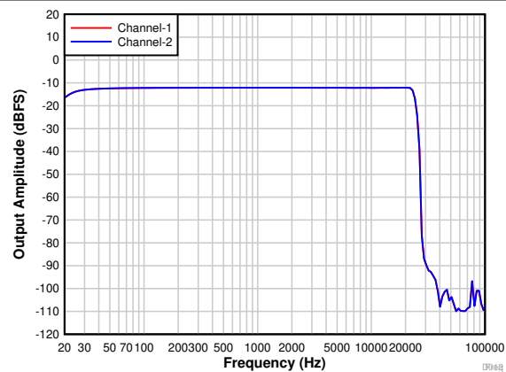
Figure 7-15. Frequency Response With a -12-dBr Input
