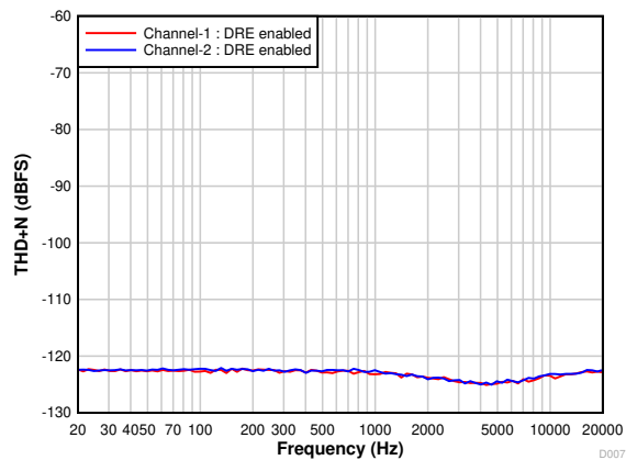
Figure 7-10. THD+N vs Input Frequency at -60-dBr Input With DRE Enabled
