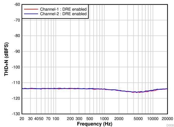
Figure 7-11. THD+N vs Input Frequency at -60-dBr Input With DRE Disabled
