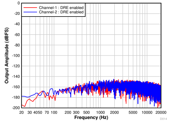
Figure 7-17. FFT With Idle Input With DRE Enabled
