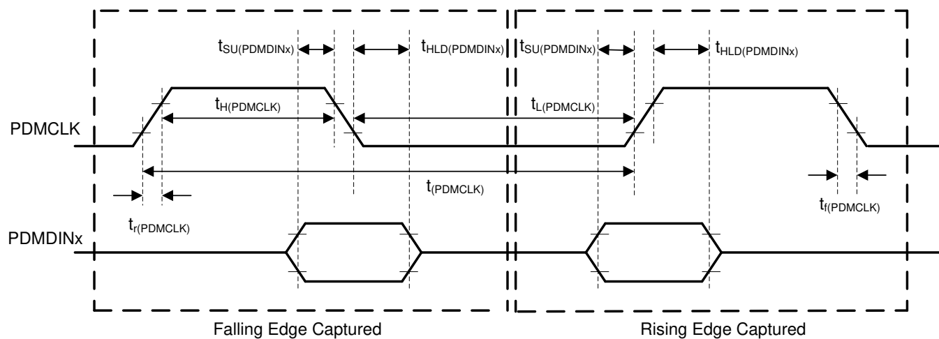
Figure 7-3. PDM Digital Microphone Interface Timing Diagram
