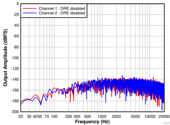
Figure 7-18. FFT With Idle Input With DRE Disabled
