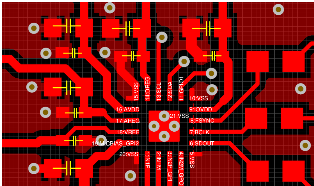
Figure 11-1. Layout Example
