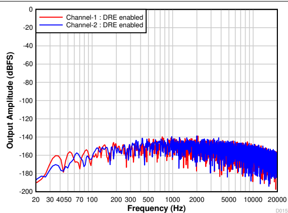
Figure 7-18. FFT With Idle Input With DRE Enabled
