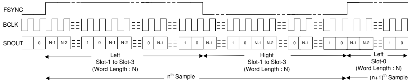
Figure 8-11. LJ Protocol Timing (No Idle BCLK Cycles, TX_OFFSET = 0)
