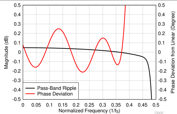
Figure 8-38. Low-Latency Decimation Filter Pass-Band Ripple and Phase Deviation
