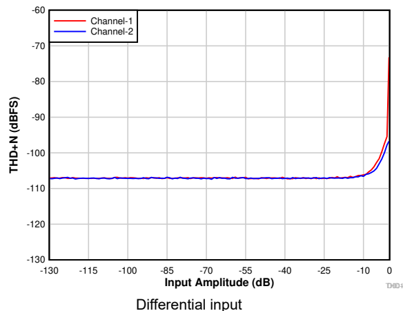
Figure 7-4. THD+N vs Input Amplitude
