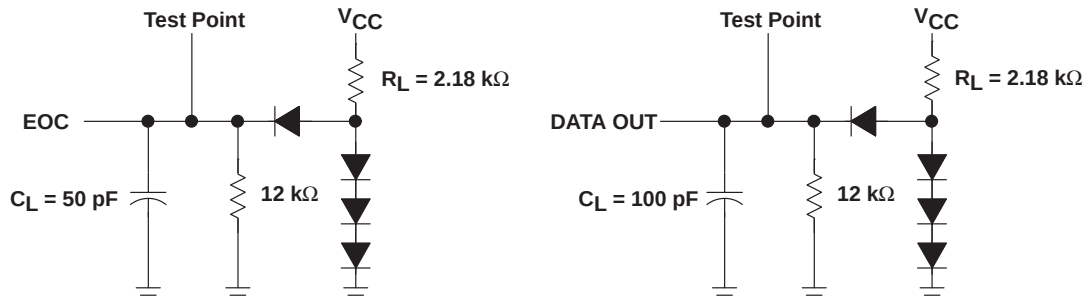
Figure 7. Load Circuits
