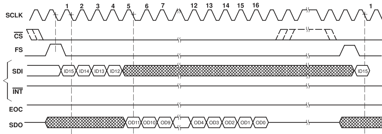
Figure 2. TLV1504/TLV1508 Read CFR Cycle (FS active)
