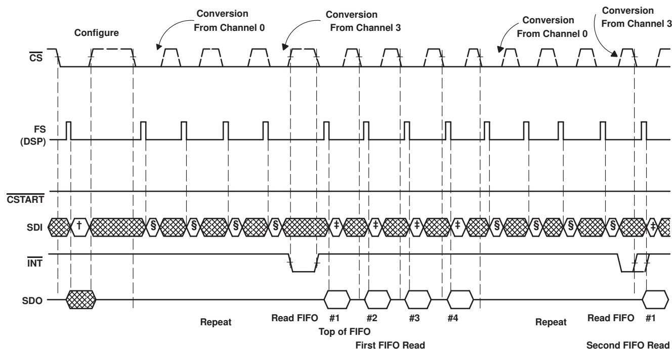
Figure 11. TLV1504/TLV1508 Mode 01 \mu\text{p/DSP} Serial Interface (Conversions Triggered by \overline{\text{CSTART}} )
