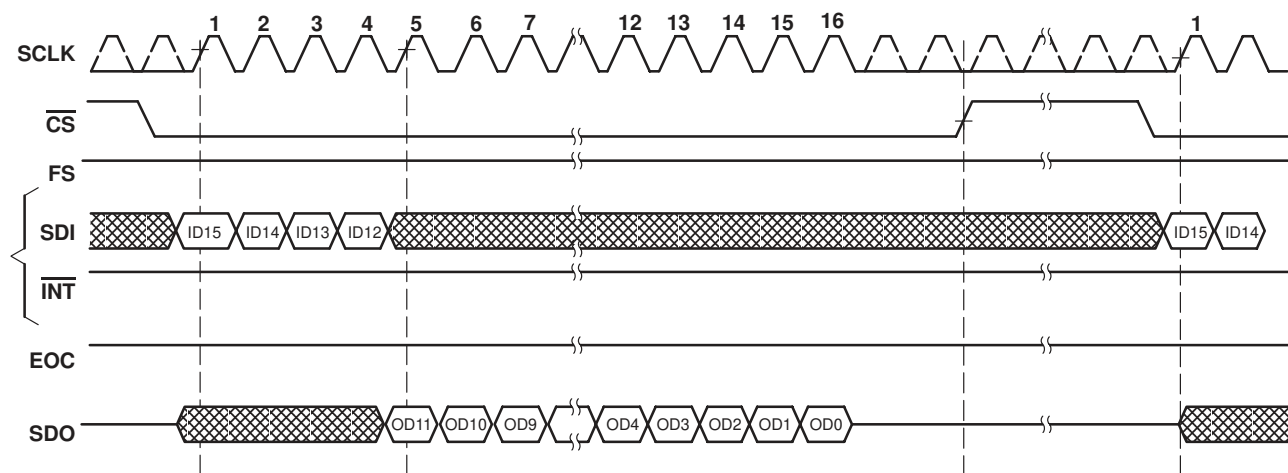
Figure 3. TLV1504/TLV1508 Read CFR Cycle (FS = 1)
