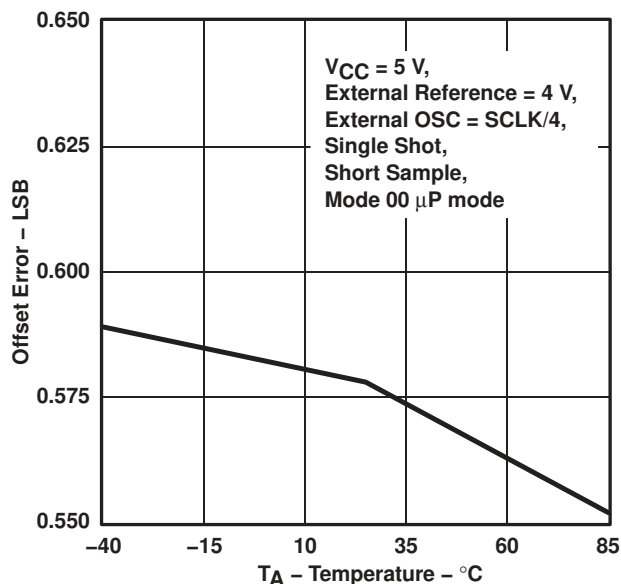
OFFSET ERROR vs TEMPERATURE
