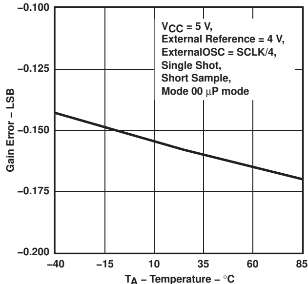
GAIN ERROR vs TEMPERATURE
