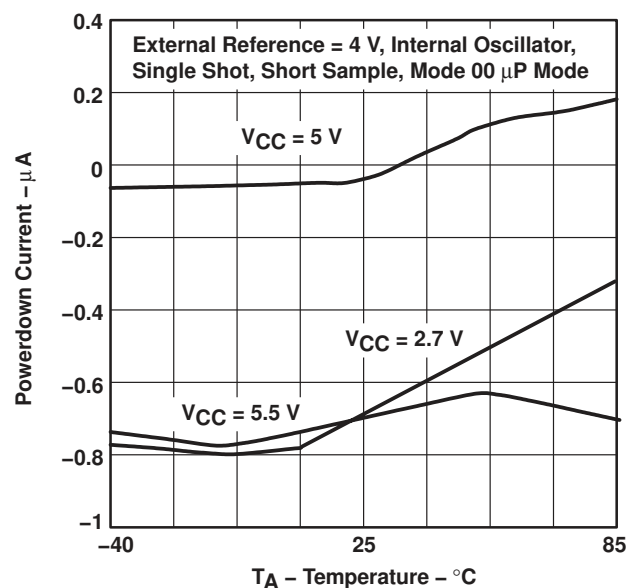
POWER-DOWN CURRENT vs TEMPERATURE
