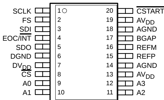
TLC3544 DW OR PW PACKAGE (TOP VIEW)
