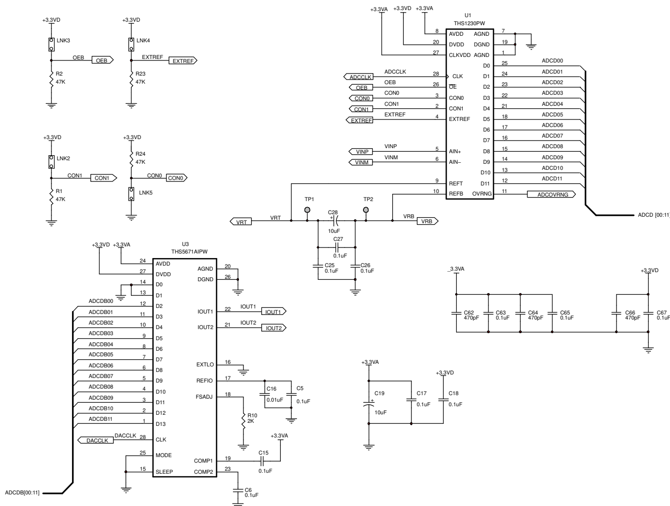
Figure 22. EVM Schematic
