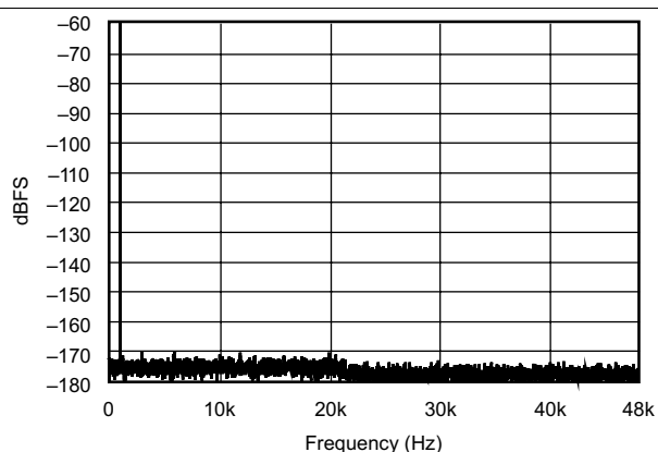
Figure 6. FFT With 1-kHz Input Tone at -60 dBFS
