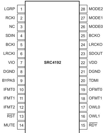
SRC4192 DB Package 28-Pin SSOP Top View
