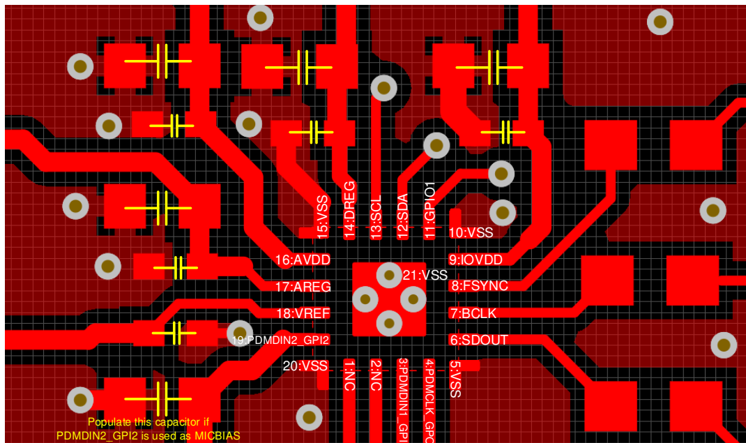
Figure 10-1. Layout Example
