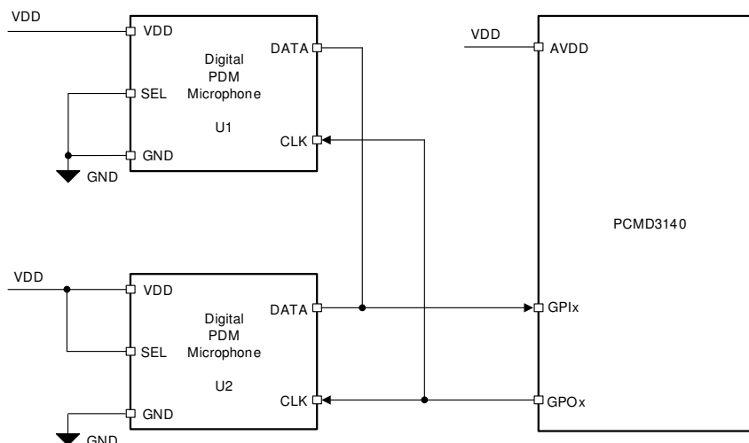
Figure 7-14. Digital PDM Microphones Connection Diagram to the PCMD3140
