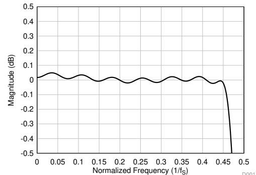
Figure 45. Linear Phase Decimation Filter Pass-Band Ripple
