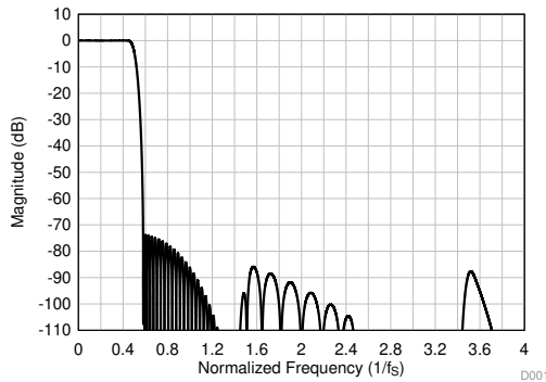
Figure 54. Linear Phase Decimation Filter Magnitude Response
