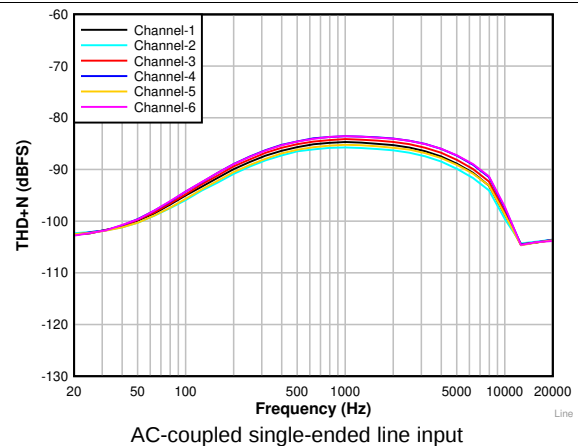
Figure 7. THD+N vs Input Frequency With a -1-dBr Input
