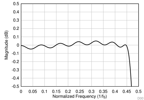
Figure 47. Linear Phase Decimation Filter Pass-Band Ripple
