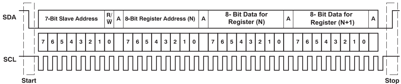
Figure 89. Typical I²C Sequence
