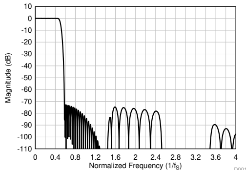
Figure 44. Linear Phase Decimation Filter Magnitude Response
