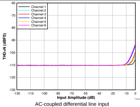
Figure 4. THD+N vs Input Amplitude
