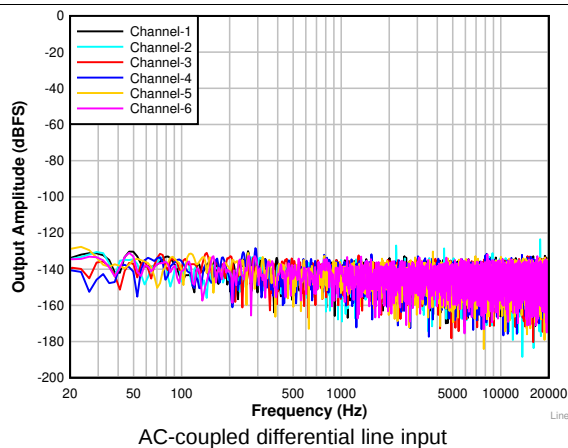
Figure 8. FFT With Idle Input
