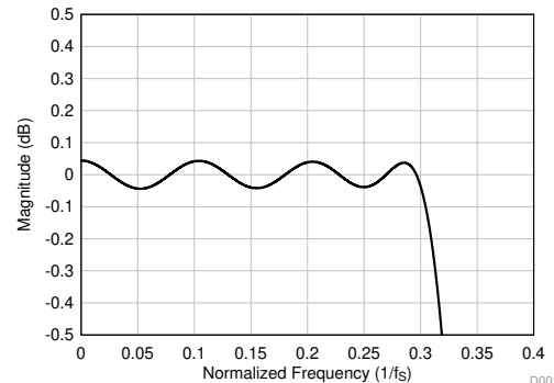
Figure 57. Linear Phase Decimation Filter Pass-Band Ripple
