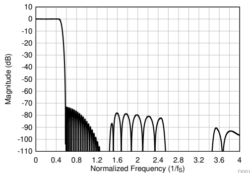
Figure 48. Linear Phase Decimation Filter Magnitude Response
