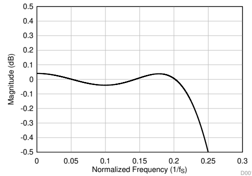
Figure 59. Linear Phase Decimation Filter Pass-Band Ripple
