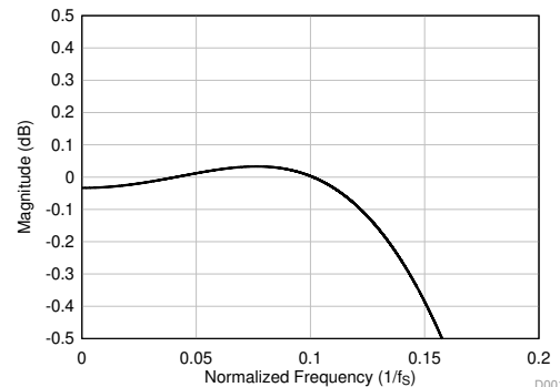
Figure 61. Linear Phase Decimation Filter Pass-Band Ripple
