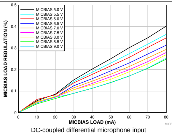
Figure 18. MICBIAS Load Regulation vs MICBIAS Load Current
