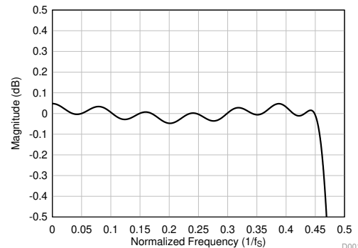
Figure 49. Linear Phase Decimation Filter Pass-Band Ripple
