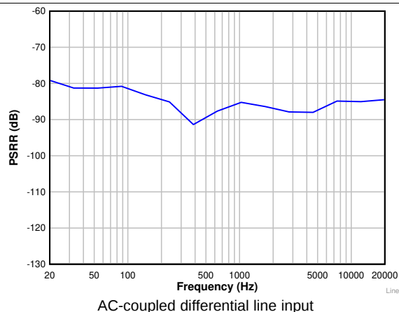
Figure 16. Power-Supply Rejection Ratio vs Ripple Frequency With 1-V pp Amplitude
