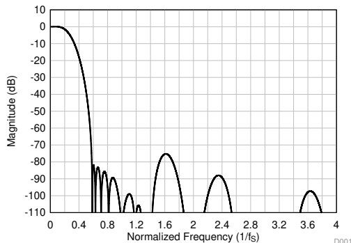
Figure 60. Linear Phase Decimation Filter Magnitude Response
