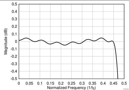
Figure 53. Linear Phase Decimation Filter Pass-Band Ripple
