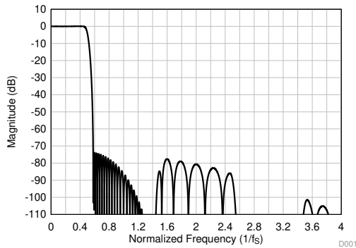
Figure 50. Linear Phase Decimation Filter Magnitude Response
