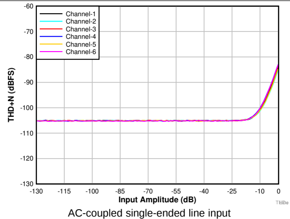
Figure 5. THD+N vs Input Amplitude
