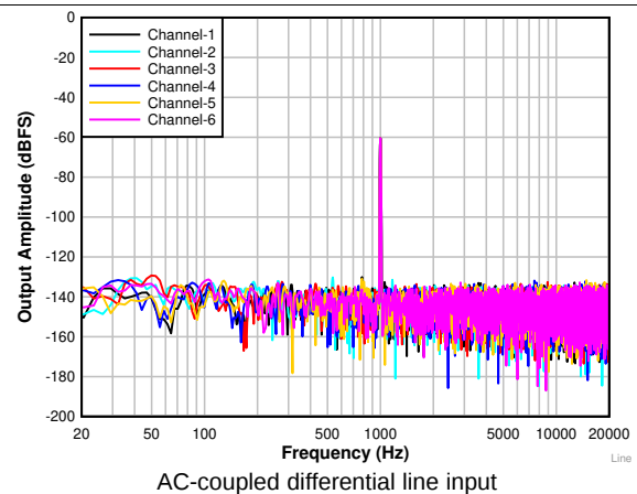
Figure 9. FFT With a -60-dBr Input
