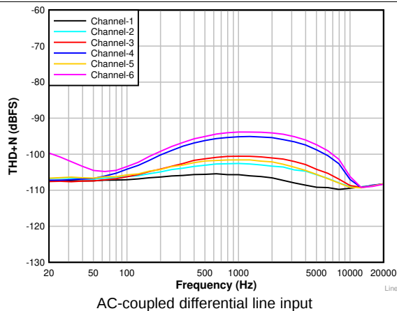
Figure 6. THD+N vs Input Frequency With a -1-dBr Input
