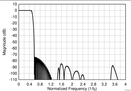
Figure 52. Linear Phase Decimation Filter Magnitude Response
