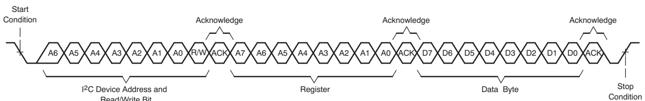
Figure 90. I²C Single-Byte Write Transfer
