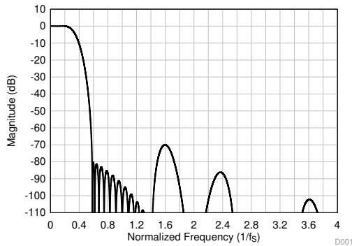
Figure 58. Linear Phase Decimation Filter Magnitude Response
