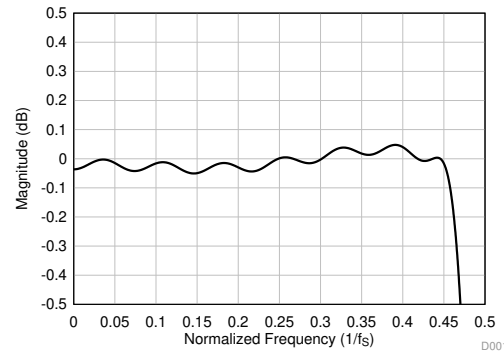
Figure 51. Linear Phase Decimation Filter Pass-Band Ripple
