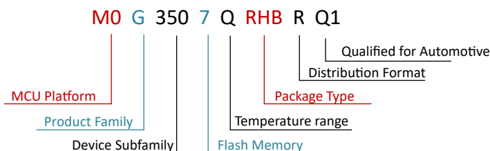
Figure 10-1. Device Nomenclature
