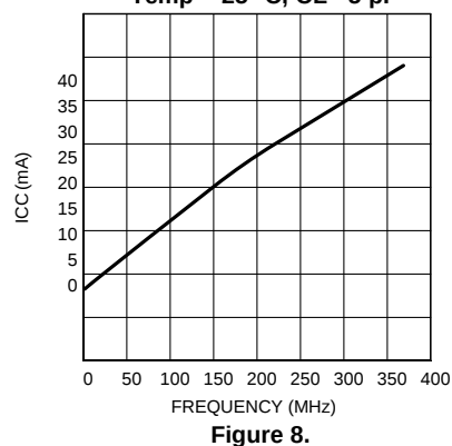
Typical Dynamic I_{CC} , LVC MOS Driver, V_{CC} = 3.3 V, Temp = 25 °C, CL = 5 pF
