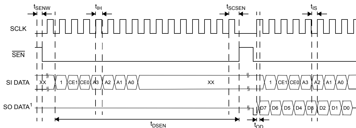
Figure 14: Serial Interface Read Command Timing
