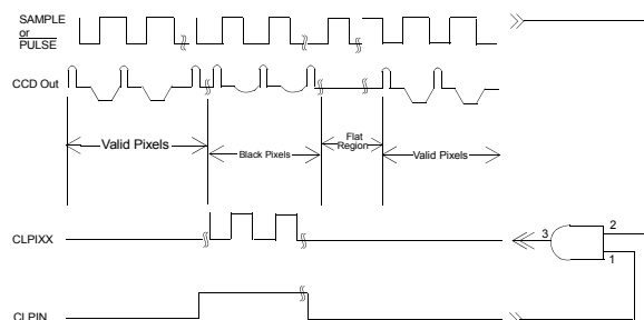
Figure 8: CLPIN gated by 'Sample' or Pulse.
