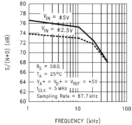
Bipolar Signal-to-Noise + Distortion Ratio vs. Input Frequency
