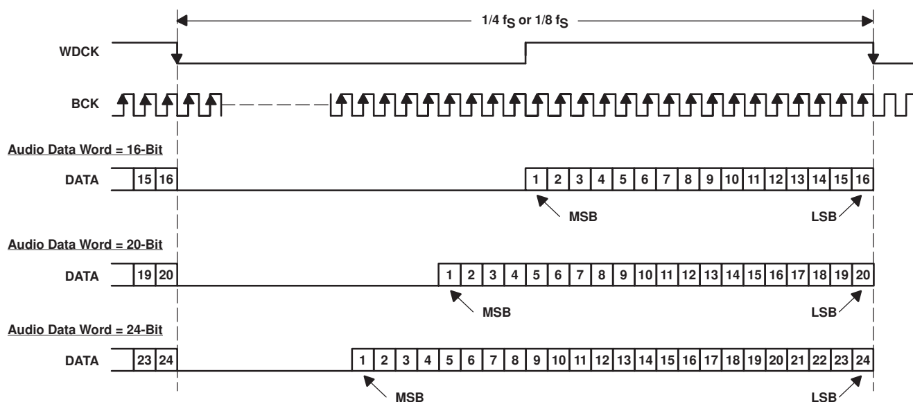
Figure 38. Audio Data Input Format for External Digital Filter (Internal DF Bypass Mode) Application
