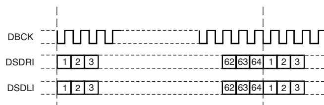
Figure 17. DSD Format
