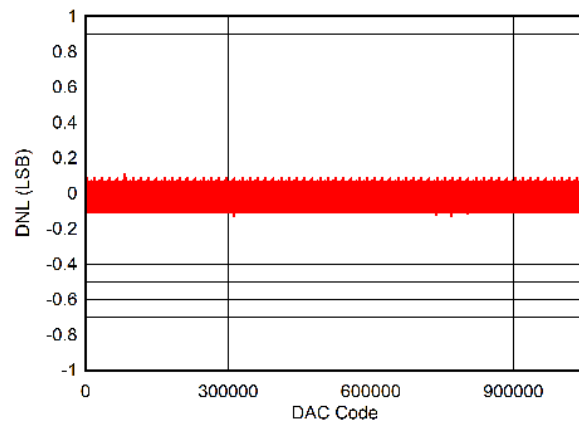
Figure 58. DNL at \pm 10 -V Output
