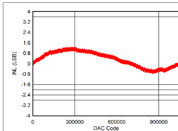
Figure 57. INL at \pm 10 -V Output
