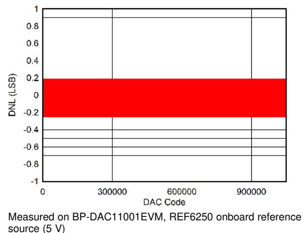
Figure 61. DNL at 0-V to 5-V Output
