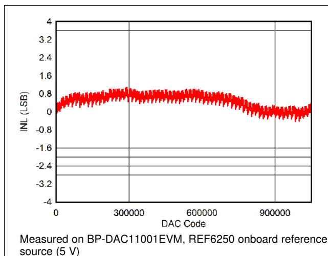
Figure 60. INL at 0-V to 5-V Output
