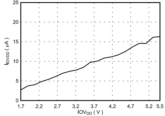
Figure 7-28. Supply Current ( IOV_{DD} ) vs Supply Voltage
