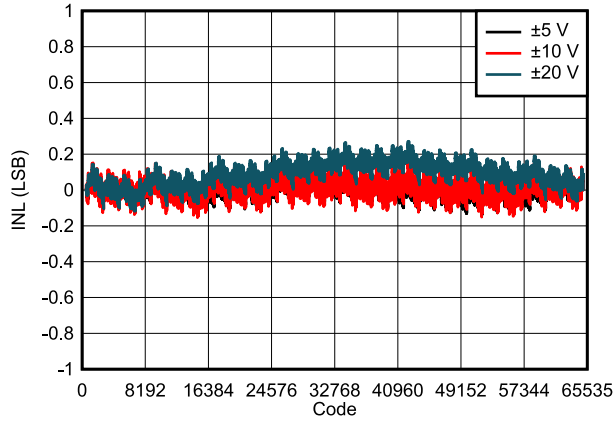
Figure 7-3. DAC81402 INL vs Digital Input Code (Bipolar Outputs)
