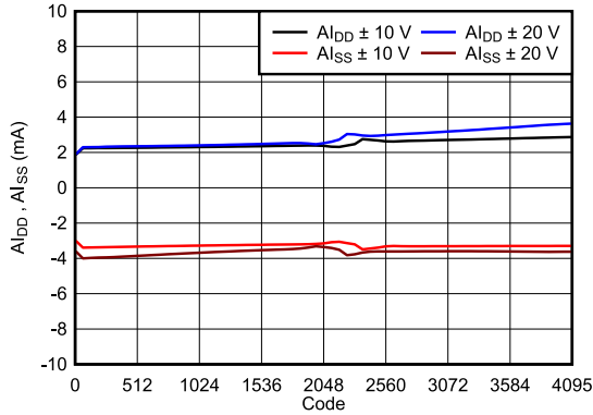
Figure 7-27. Supply Current ( Al_{DD} , Al_{SS} ) vs Digital Input Code
