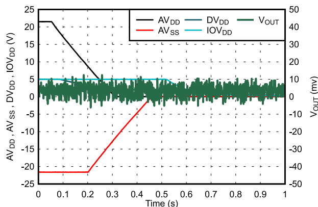
Figure 7-39. Power-Down Response
