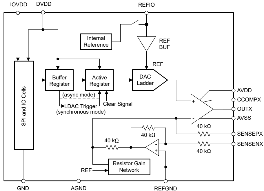
Figure 8-1. Device Architecture
