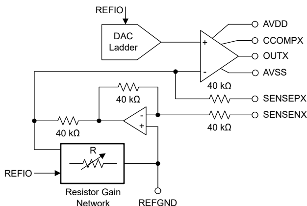
Figure 8-3. Voltage Output Buffer
