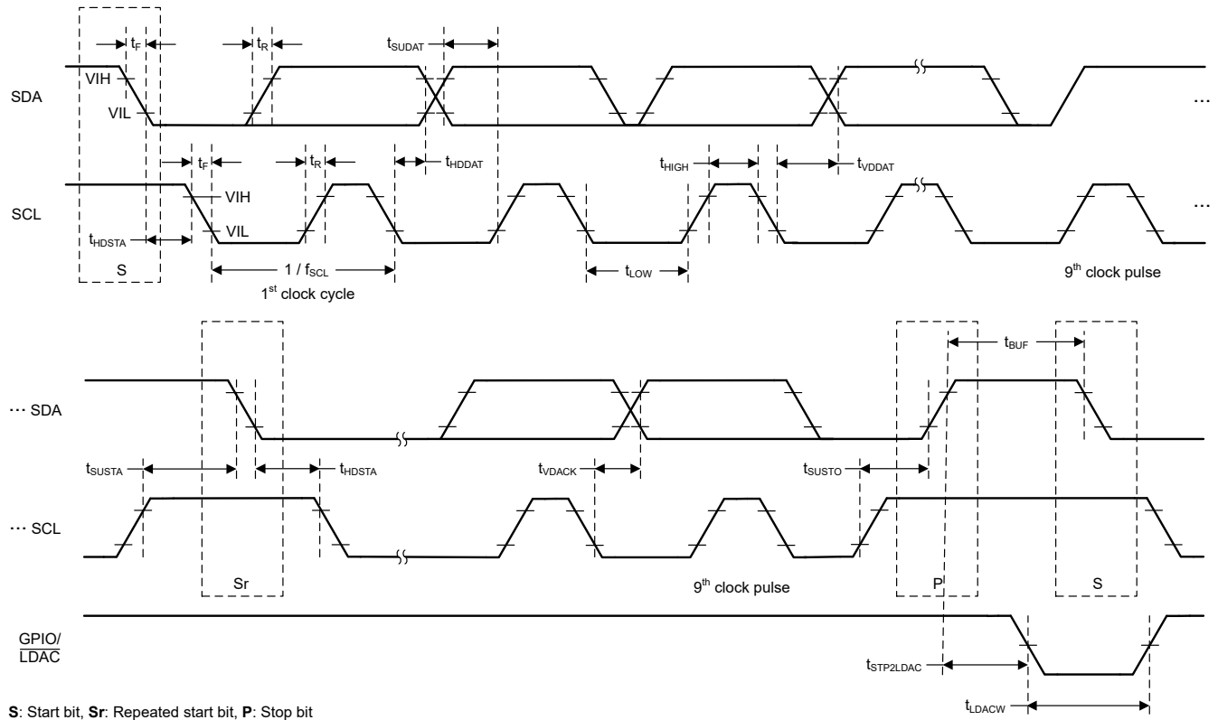
Figure 5-1. I²C Timing Diagram
