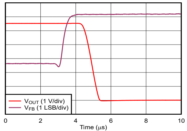
Figure 5-52. Comparator Response Time: High-to-Low Transition
