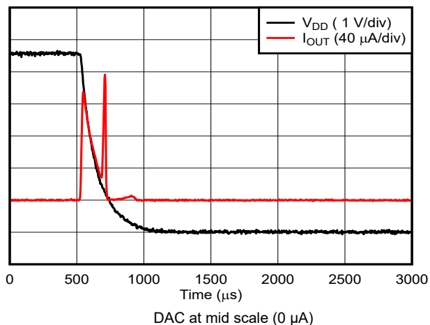
Figure 6-52. Current Output Power-Off Glitch
