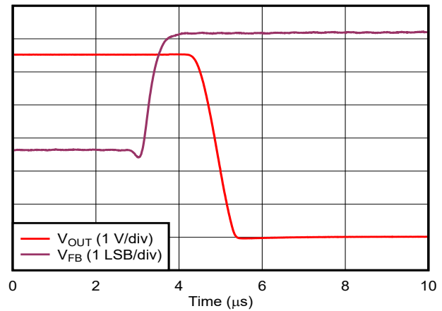
Figure 6-60. Comparator Response Time: High-to-Low Transition
