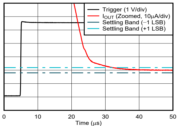
Figure 6-50. Current Output Setting Time, Falling Edge
