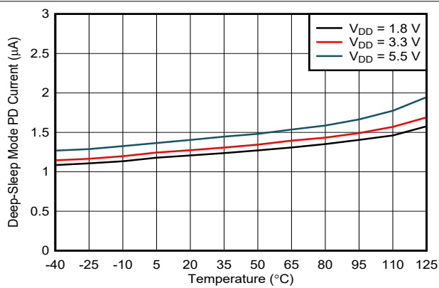
Figure 6-65. Power-Down Current vs Temperature
