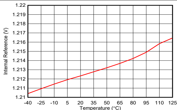
Figure 6-62. Internal Reference vs Temperature
