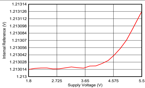
Figure 6-63. Internal Reference vs Supply Voltage
