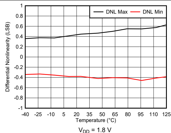
Figure 5-10. Differential Nonlinearity vs Temperature
