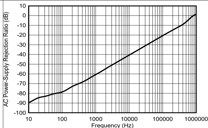
Figure 5-43. AC Power-Supply Rejection Ratio vs Frequency
