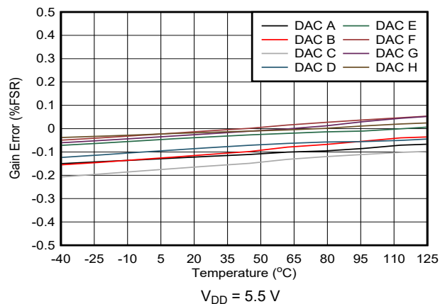
Figure 5-29. Gain Error vs Temperature
