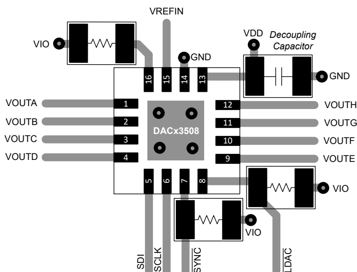
Figure 8-5. Layout Example
