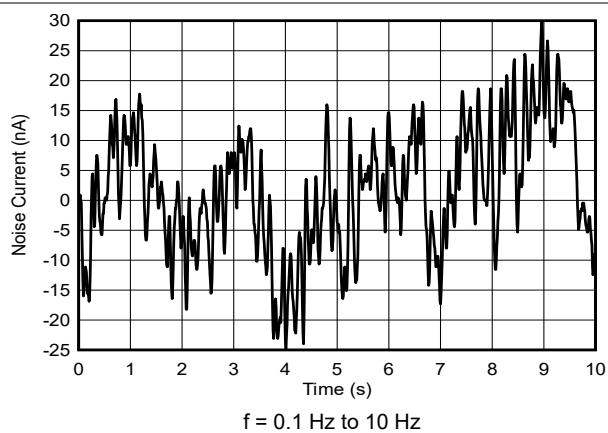
Figure 5-50. Current Output Flicker Noise
