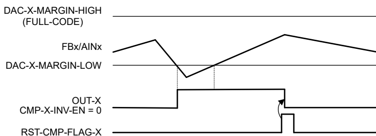
Figure 6-7. Latching Comparator With Active High Output
