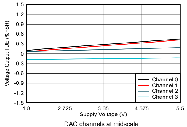
Figure 5-15. Voltage Output TUE vs Supply Voltage
