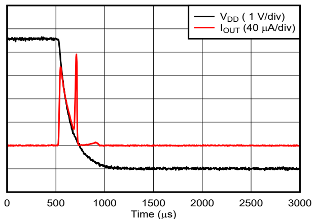
Figure 6-50. Current Output Setting Time, Falling Edge
