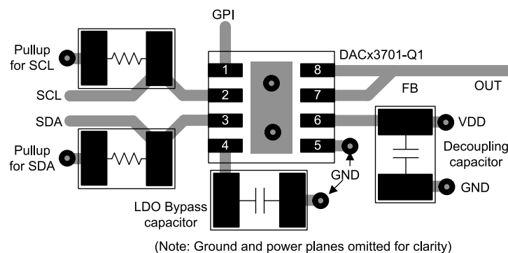
Figure 8-6. Layout Example
