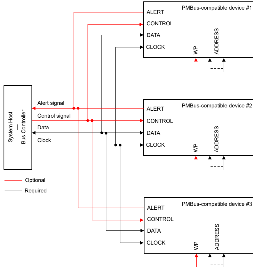
Figure 7-2. PMBus Connections
