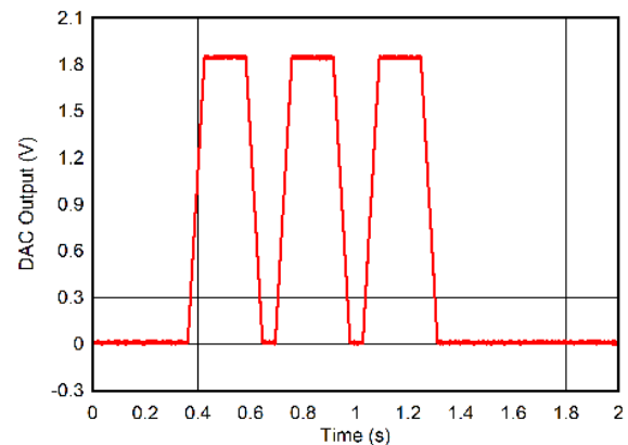
Figure 9-9. Medium Priority Alarm
