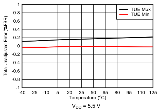
Figure 5-17. Total Unadjusted Error vs Temperature
